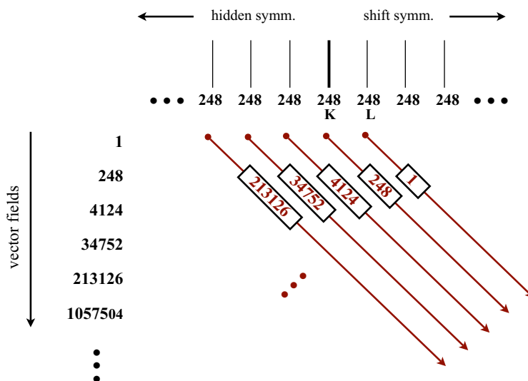
Figure 1: Couplings induced by different components of the embedding tensor \Theta_{\mathcal{M}} .
